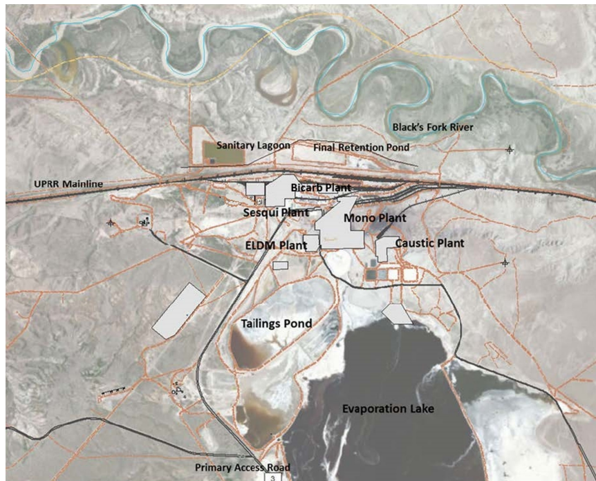
Figure 2.4 Westvaco Surface Production Facilities
