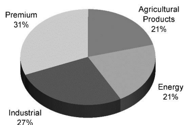
2018 Freight Revenue
