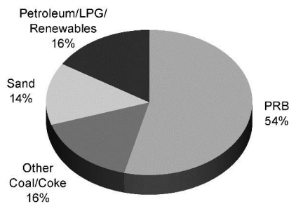
2018 Energy Carloads
