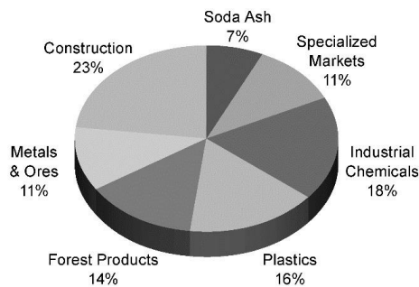
2018 Industrial Carloads
